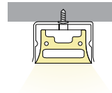
CURVED STAINLESS STEEL PROFILE FOR 20×14mm NEON LIGHT 1m SKU: E9010803-026
