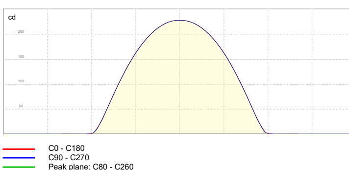
LINEAR INTENSITY DISTRIBUTION DIAGRAM
