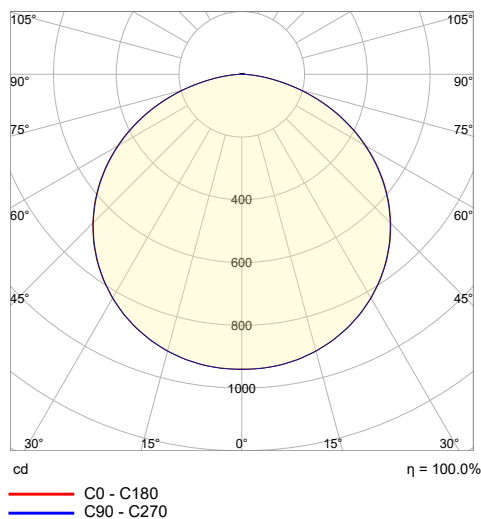
POLAR GRAPH - MAIN PLANES
