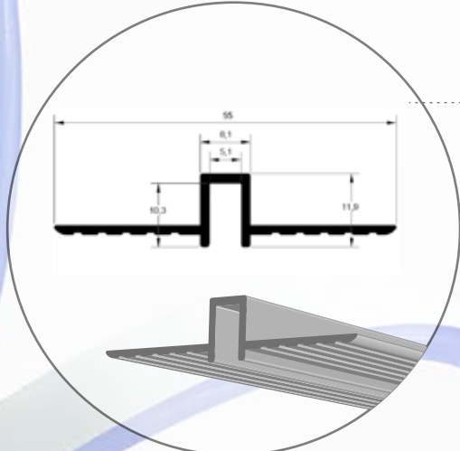
ALUMINUM PROFILE Π FOR 6X12 NEON LIGHT
