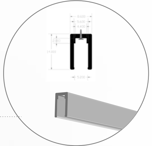
CLIP FOR NEON STRIP 6MM PVC 5CM PC
